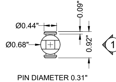
2 TENSION FORK - END VIEW SCALE = 1:2
