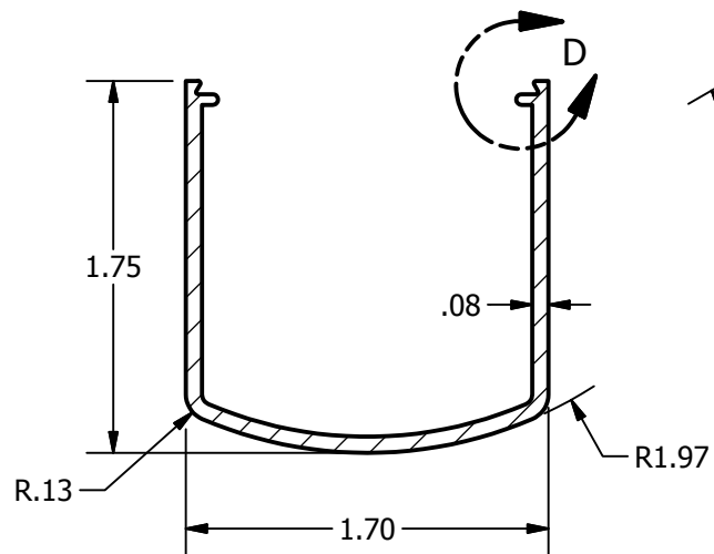
SECTION C-C SCALE 1 : 1
