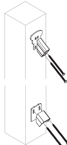
UPPER NEWEL POST (Figure 2.1)
