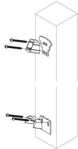
LOWER NEWEL POST (Figure 2.2)
