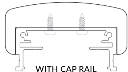
WITH CAP RAIL (cap rail not included)
